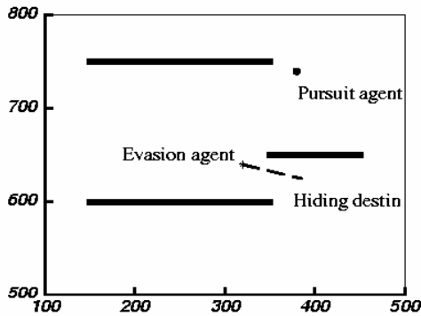
(b) Overcoming the masking effect in hiding.
