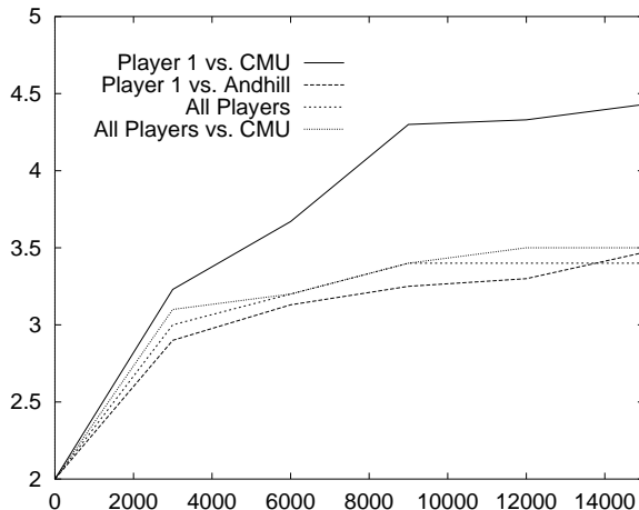
Figure 3. Player 1 (forward) against CMUnited97 contrasted with Player 1 against Andhill97 under same input condition. Means across all players provided for comparison.
