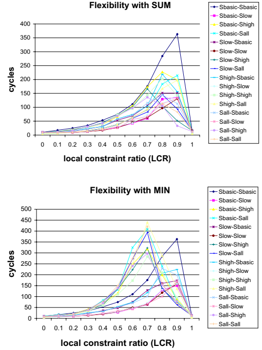
Figure 5: Comparing NVA strategies: cycles
