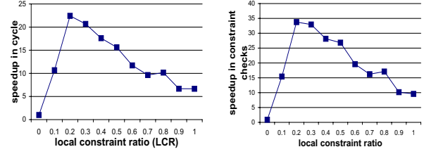
(a) negotiation cycle (b) constraint checks Figure 7: Performance improvement from Argumentation.
