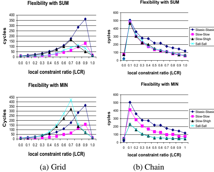
(a) Grid (b) Chain Figure 6: Comparing NVA strategies: negotiation cycles
