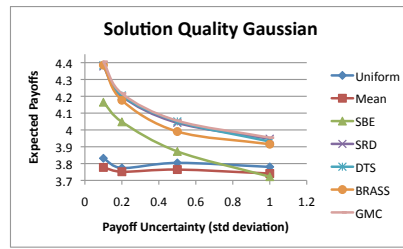
(b) Solution quality comparison for infinite games with Gaussian attacker payoff distributions with identical standard deviations.
