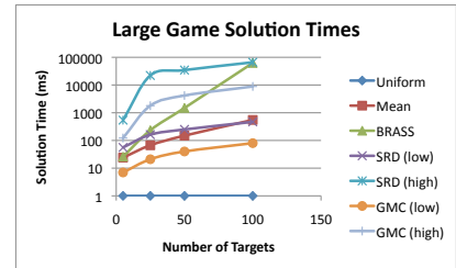
(f) Computational cost comparison for solving large game instances of Gaussian variable games.
