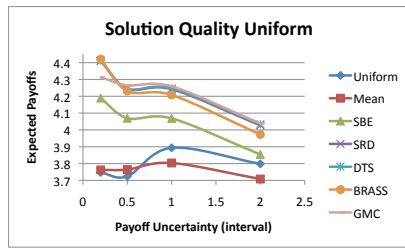
(a) Solution quality comparison for infinite games with uniform attacker payoff distributions.
