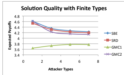
(d) Solution quality results for small games with a finite set of known attacker types.
