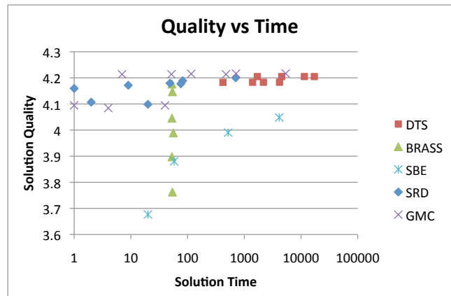
Figure 3: Comparison of the tradeoff in solution quality and computational cost for each of the algorithms, exploring the effects of different parameter settings.
