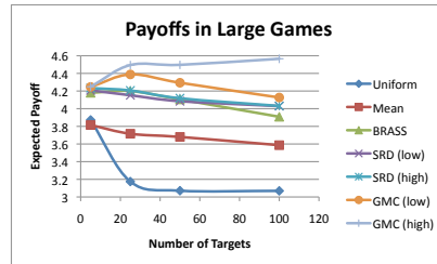
(e) Solution quality results when scaling to larger game instances for Gaussian attacker payoff distributions with varying standard deviations.
