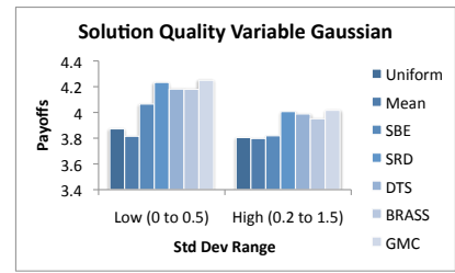
(c) Solution quality comparison for infinite games with Gaussian attacker payoff distributions with varying standard deviations.
