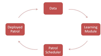
Figure 2: Scheduler flowchart
