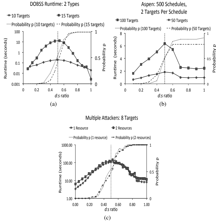
Fig. 8 Average runtime for computing the optimal solution for an example setting for all the three security domains, along with the probability p plotted on the secondary y-axis. The vertical dotted line shows d:s = 0.5 .
